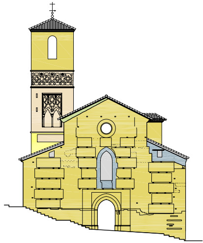
Alzado principal
